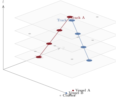
Fig. 3 Identity tubes in spatio-temporal space. Each vessel forms a coherent “tube” through (x, y, t) space as ST-DBSCAN links detections across frames. Isolated clutter points (gray) lack temporal continuity and are rejected as noise.
